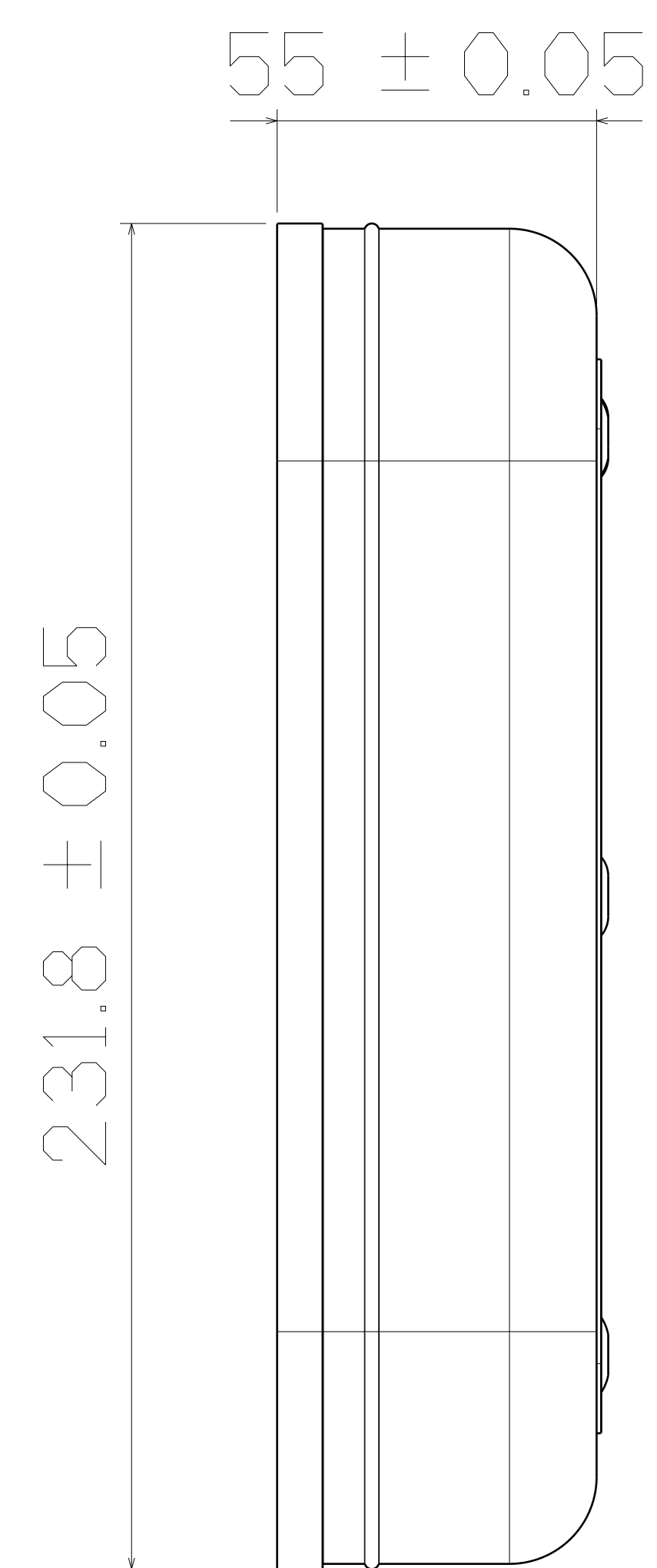
RIGHT VIEW
