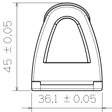
RIGHT VIEW
