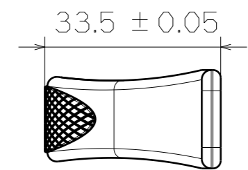
RIGHT VIEW
