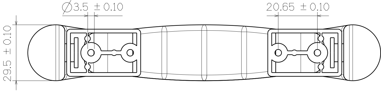
BOTTOM VIEW
