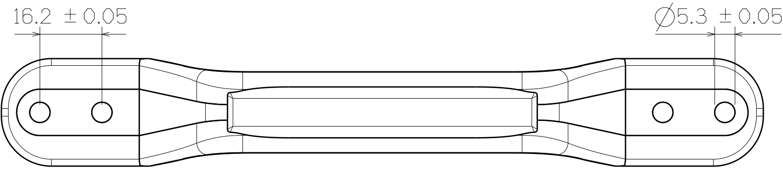
TOP VIEW
