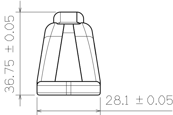
RIGHT VIEW
