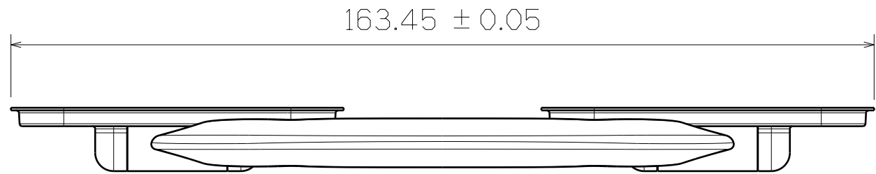
TOP VIEW
