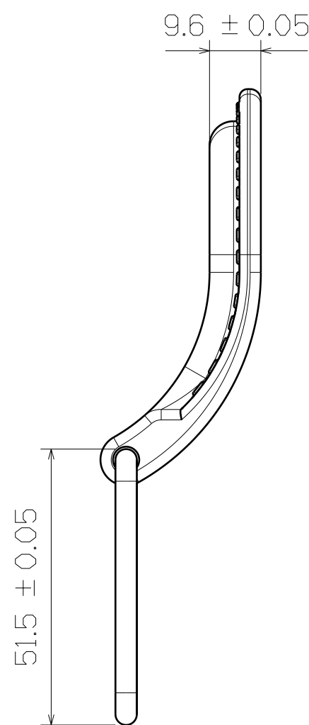
RIGHT VIEW
