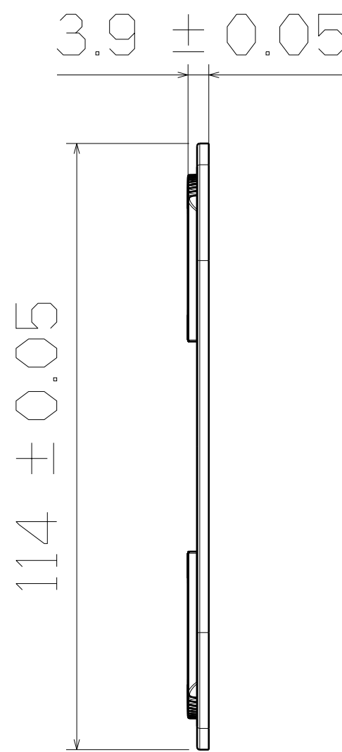
Right View
