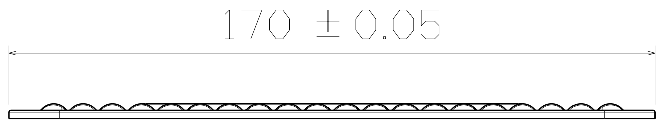
Top View
