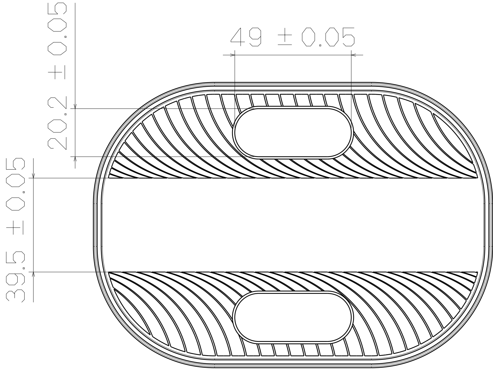
Top View
