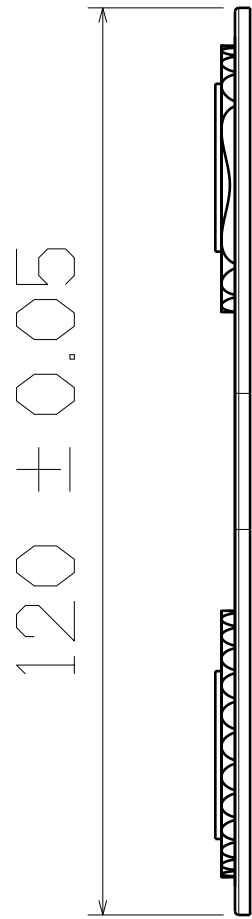
Right View
