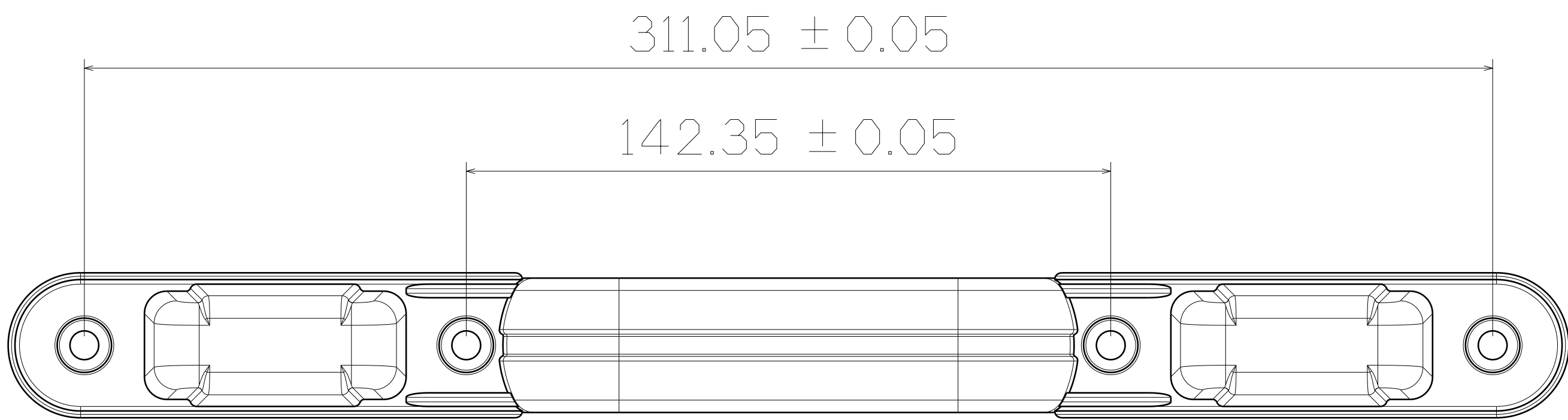
Top View
