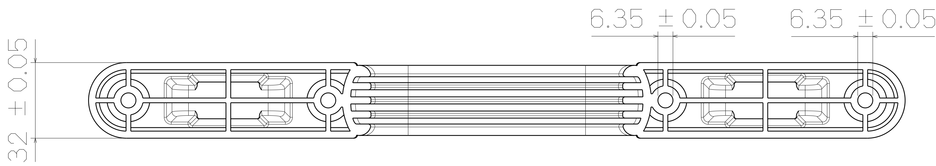
Bottom View
