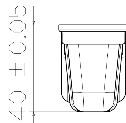
Right View
