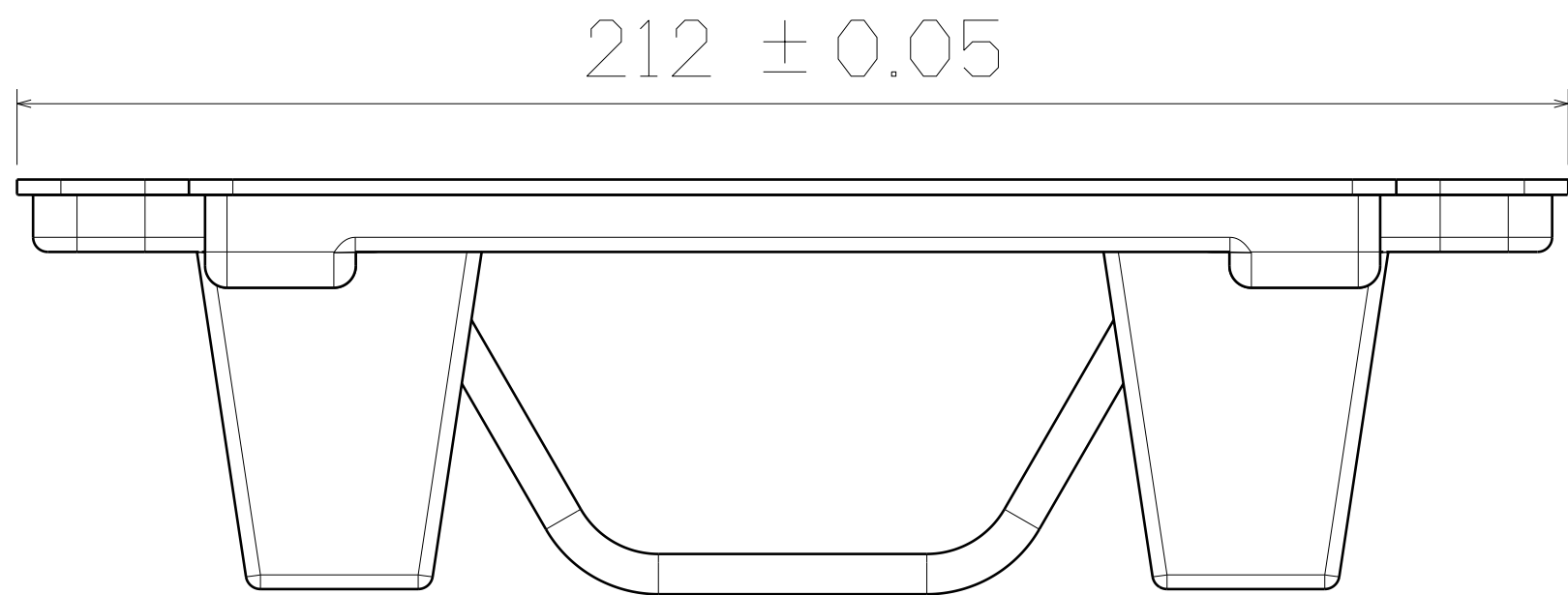
TOP VIEW
