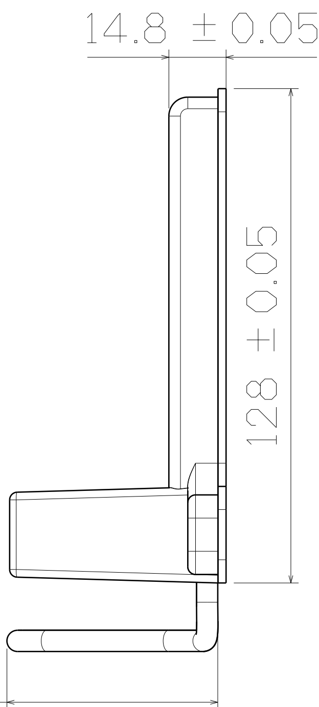
RIGHT VIEW
