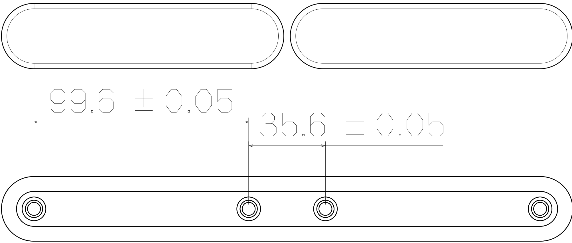
BACK VIEW
