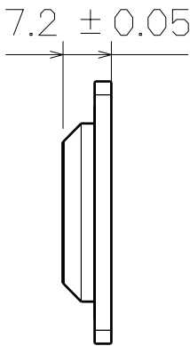
Right View
