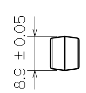
RIGHT VIEW
