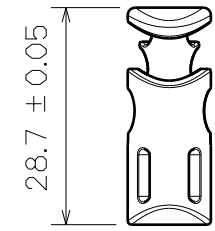
Right View
