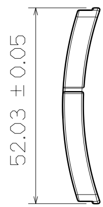
Right View
