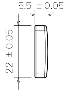
RIGHT VIEW
