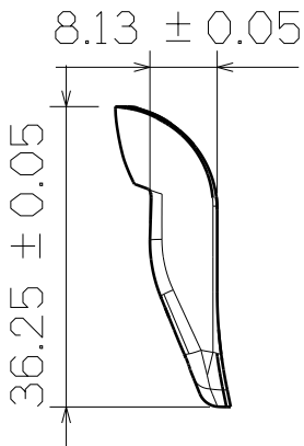
Right View
