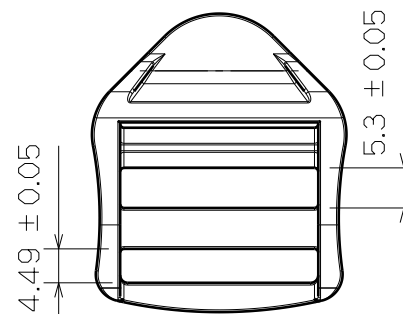
Back View
