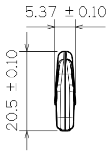
Right View
