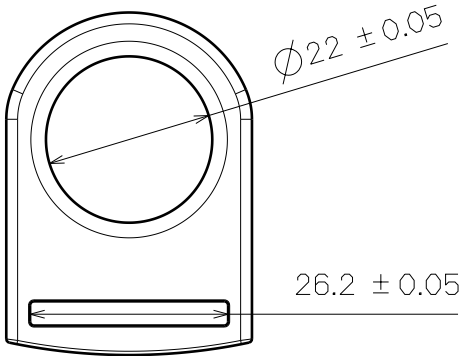
SF439 WEBBING END FRONT VIEW
