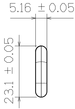
RIGHT VIEW
