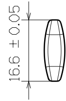
Right View
