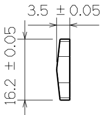
Right View
