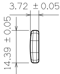
Right View
