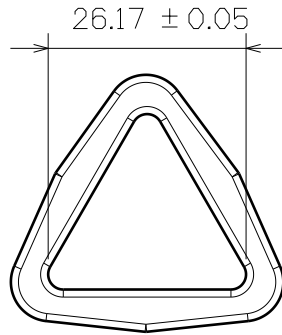
SF414-25mm
