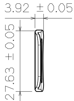
Right View
