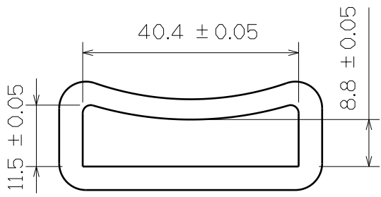
SF406-2-38mm
