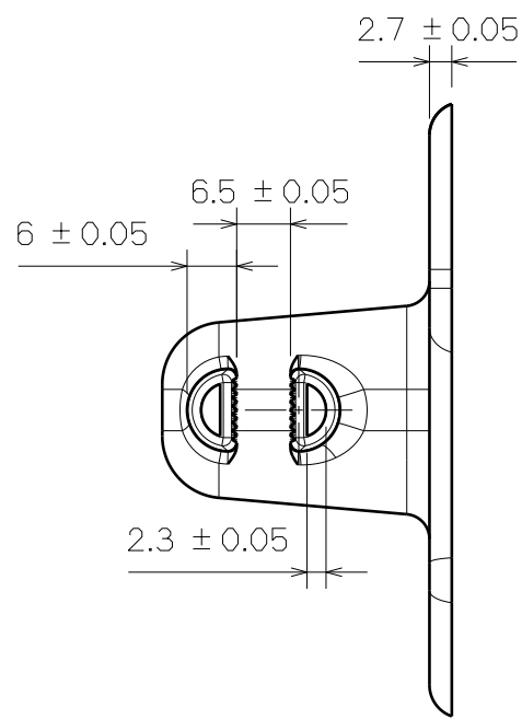
Right View
