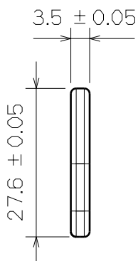
Right View
