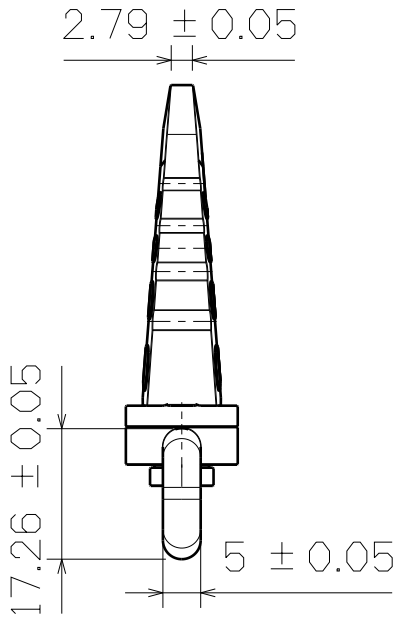
Right View
