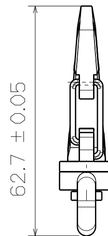
Left View
