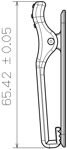
Right View
