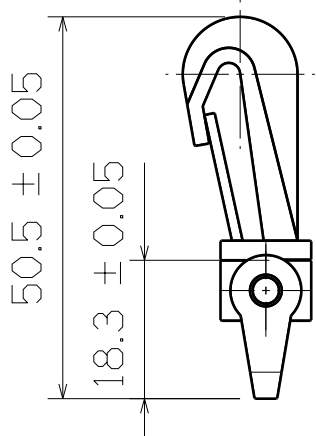
Right View
