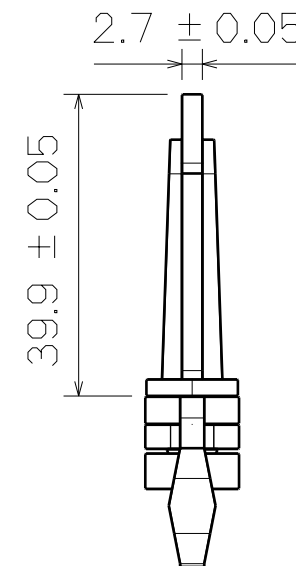
Left View
