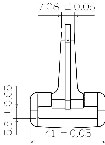
Right View
