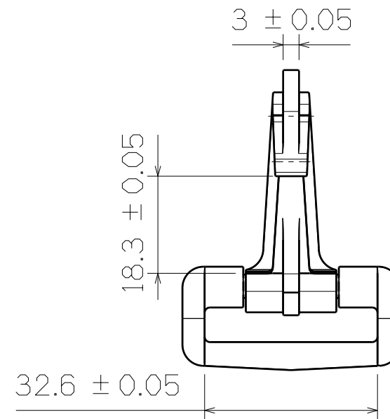
Left View
