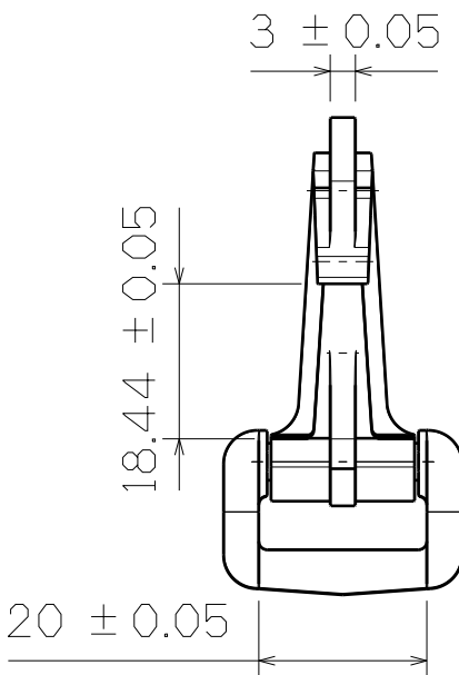
Left View
