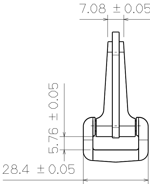
Right View
