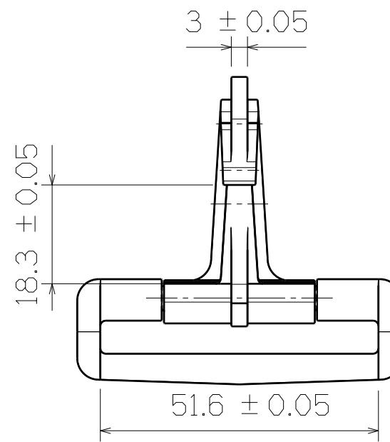
Left View
