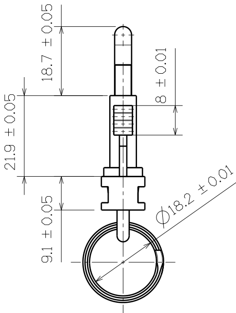
Left View
