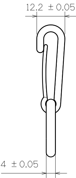
Right View
