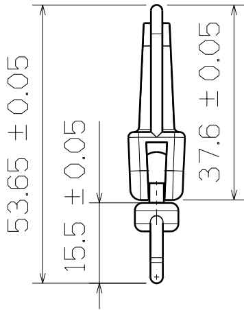
Right View
