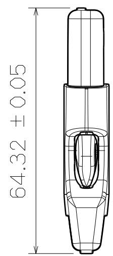
Right View
