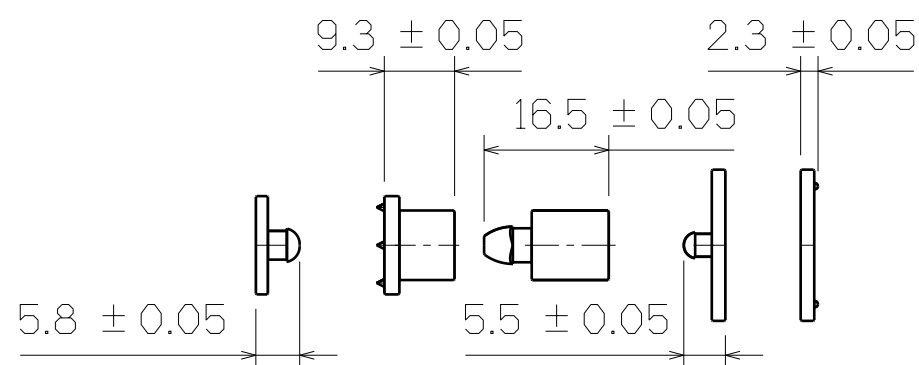
Right View
