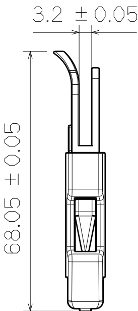
Right View
