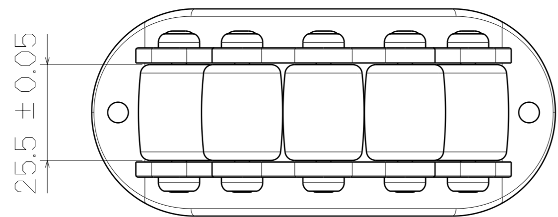
Top View
