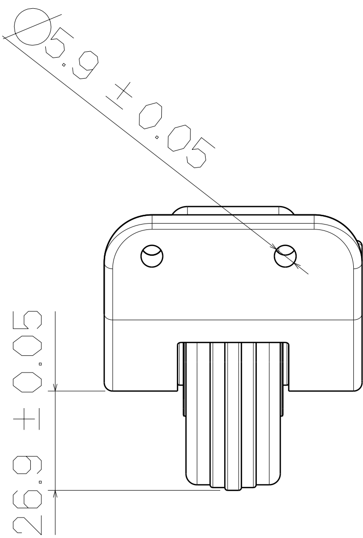
LEFT VIEW
