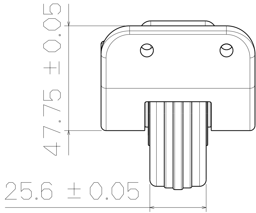
RIGHT VIEW
