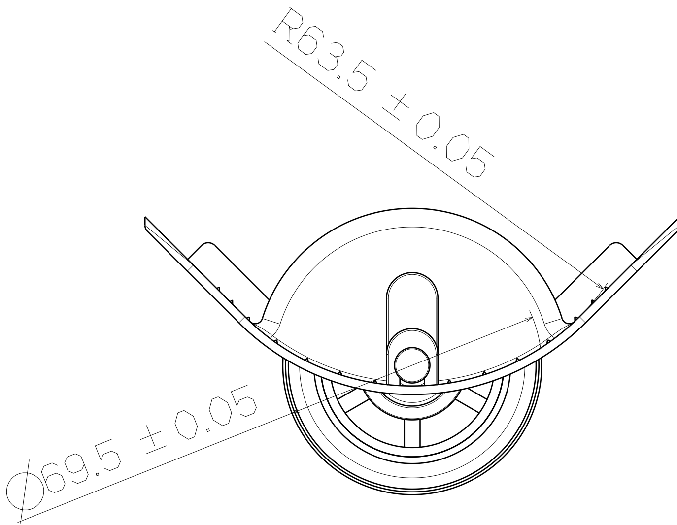
BACK VIEW
