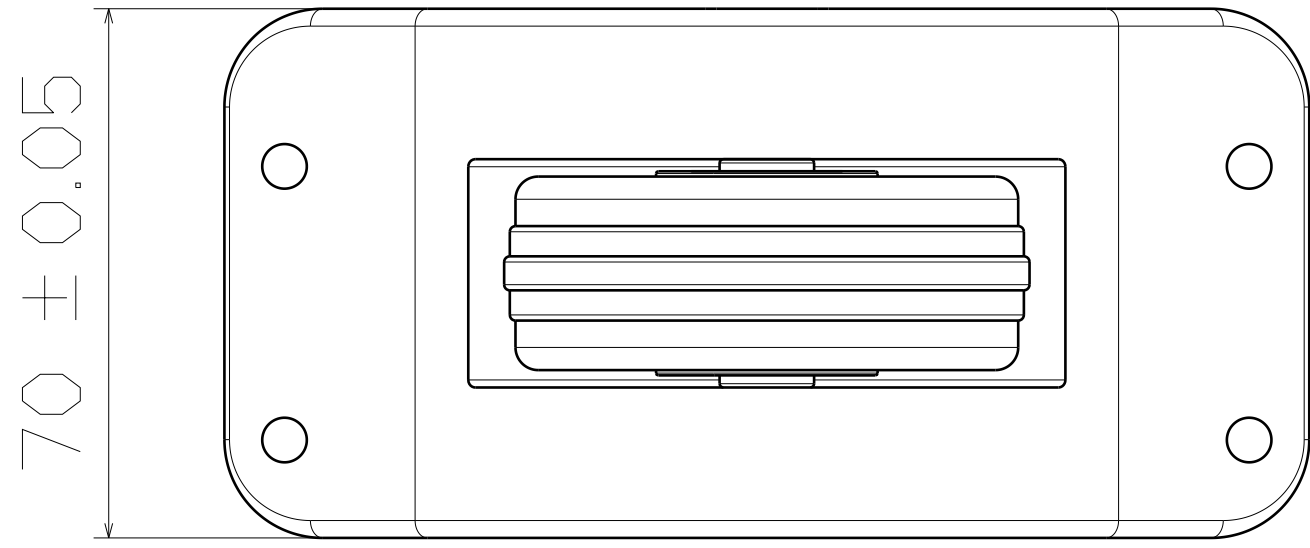
BOTTOM VIEW
