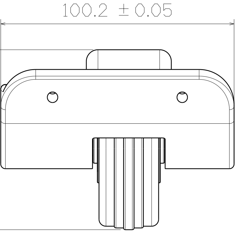
Right View
