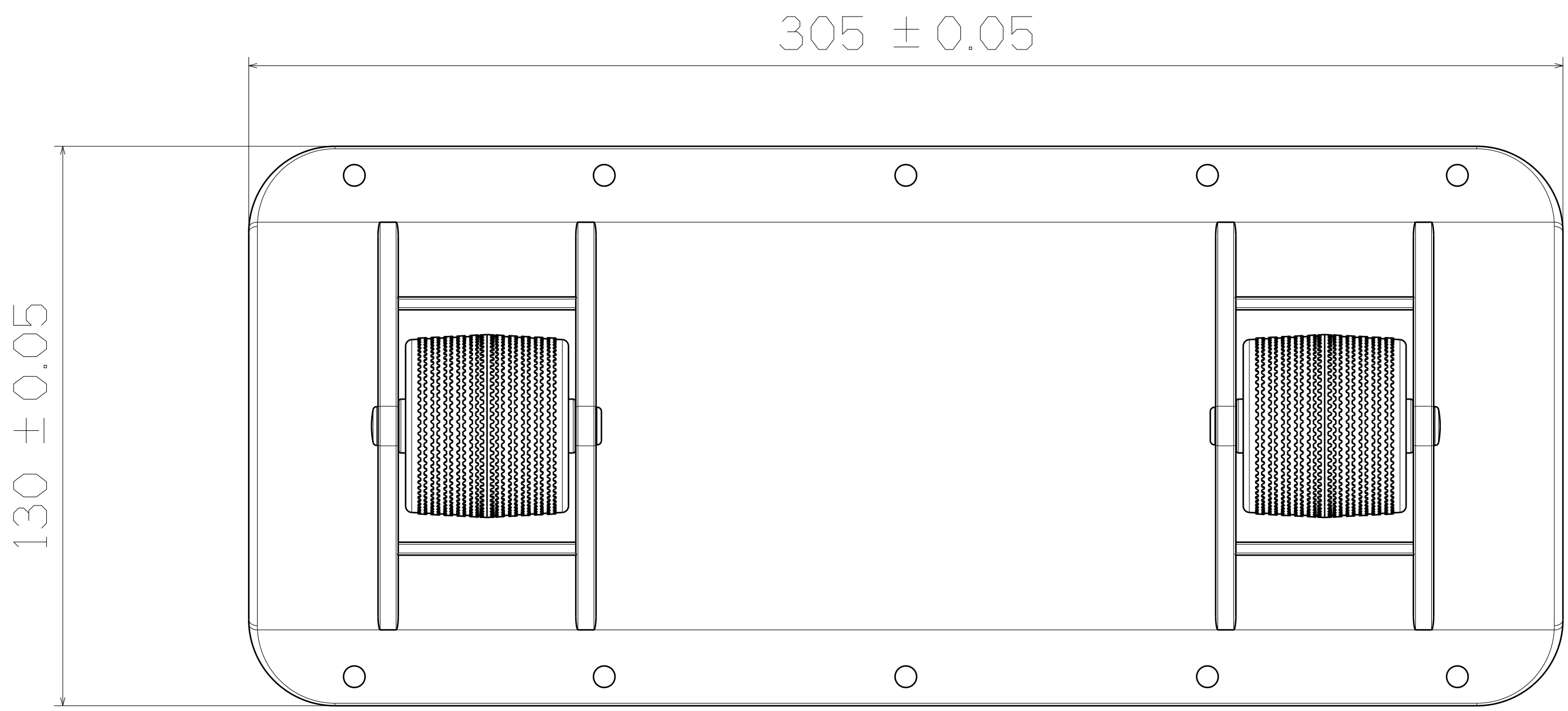
Top View
