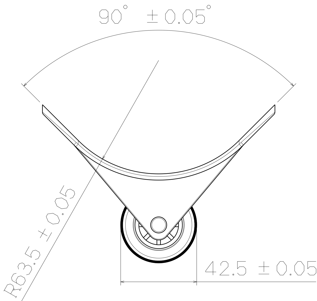
Right View
