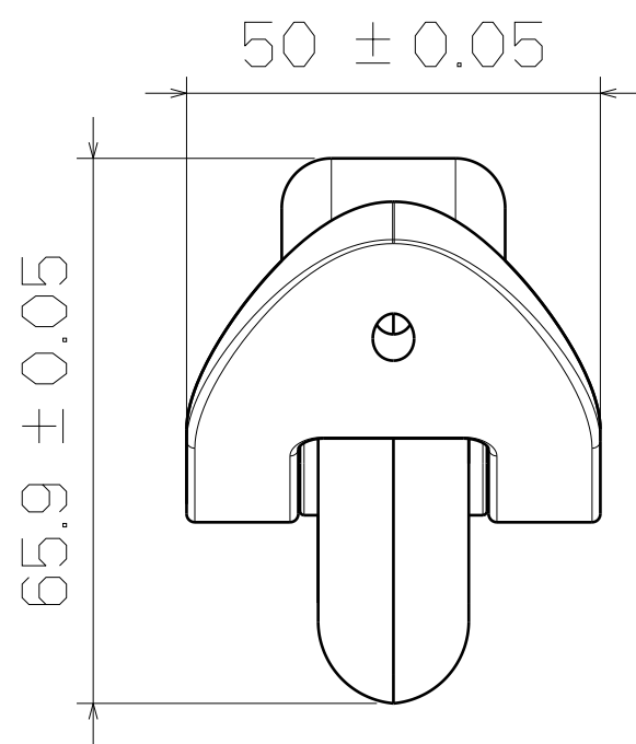
Right View
