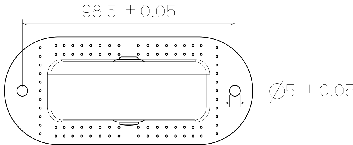
Bottom View
