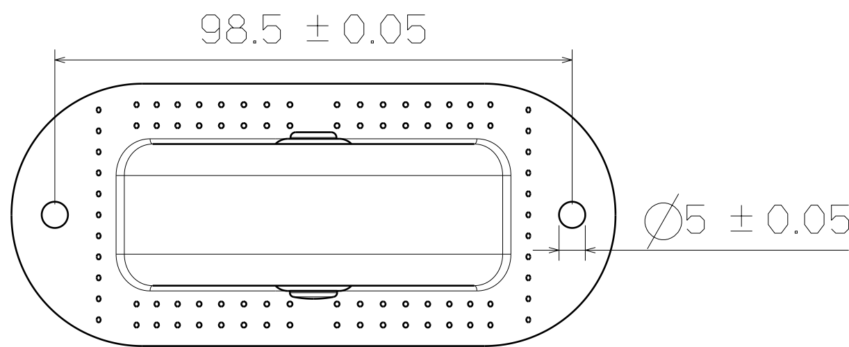
Bottom View
