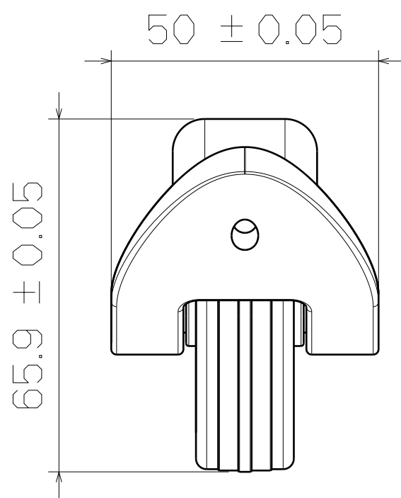
Right View
